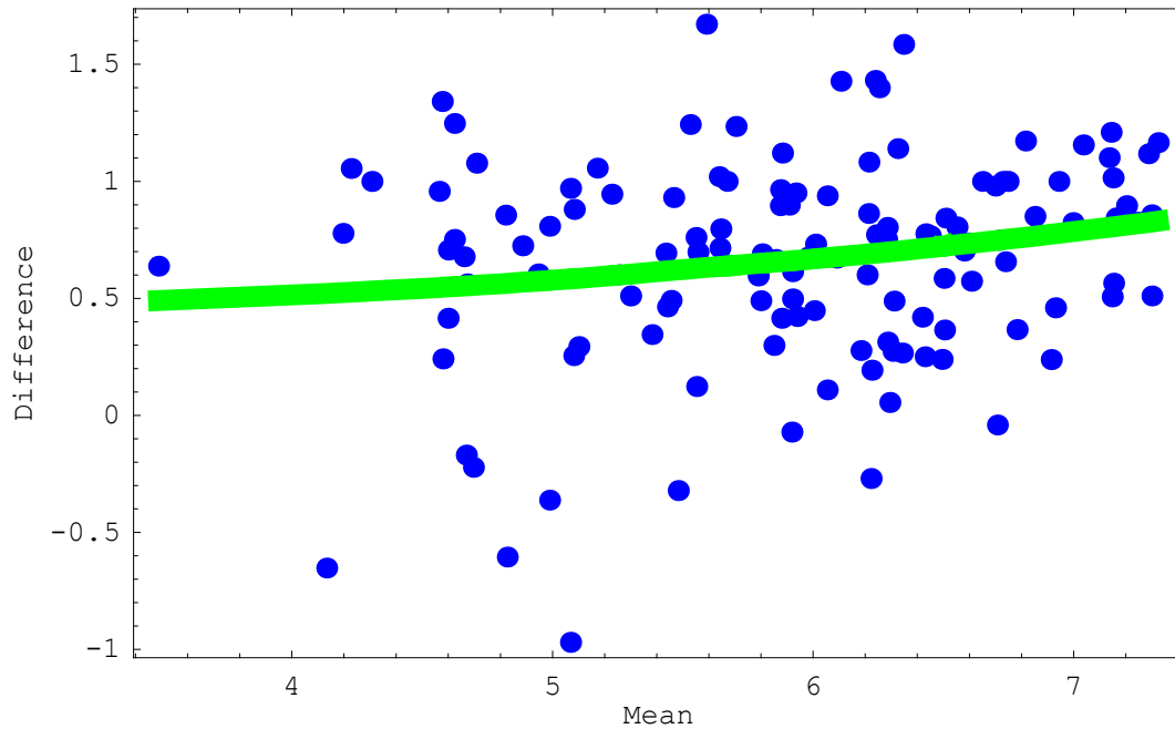
Figure 1. Tukey mean-difference plot of ozone pollution at Stamford and Yonkers.
