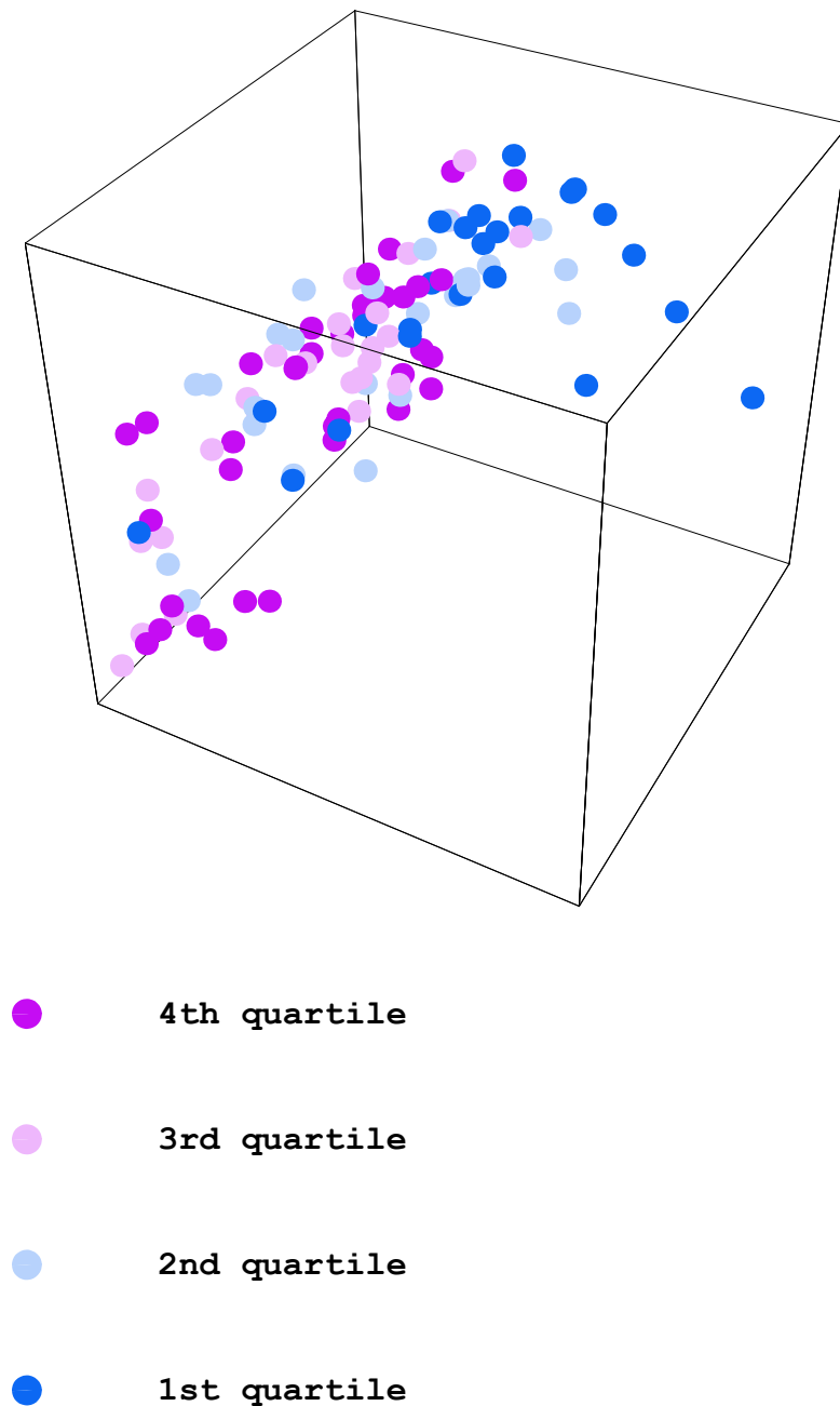
Figure 3. 3D Scatterplot of environmental data ( W , wind; T_p temperature; R radiation) and ozone (cube-root, color coded).
