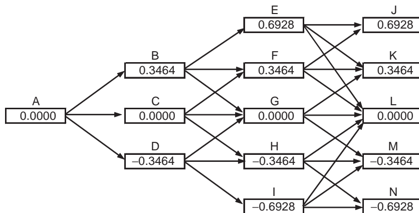
Figure 33.1 Tree for X . Constructing this tree is the first stage in constructing a tree for the spot price of a commodity, S . Here p_u , p_m , and p_d are the probabilities of “up”, “middle”, and “down” movements from a node.
