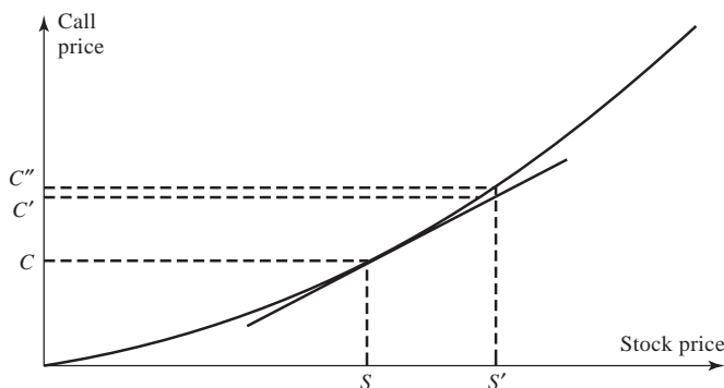
Figure 18.7 Hedging error introduced by nonlinearity.
